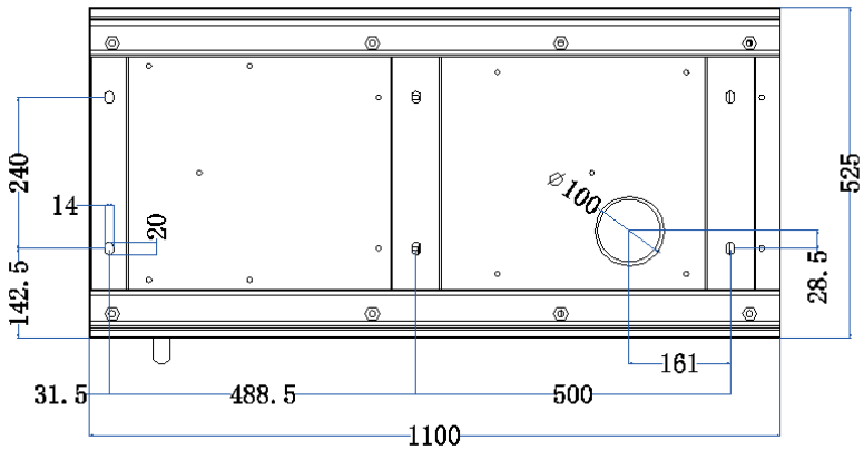
Base anchoring hole diagram
